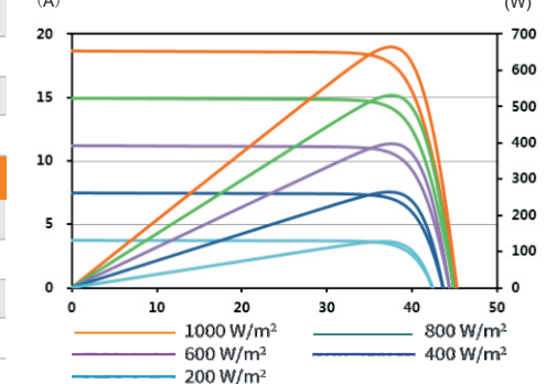
Current-Voltage Curve
