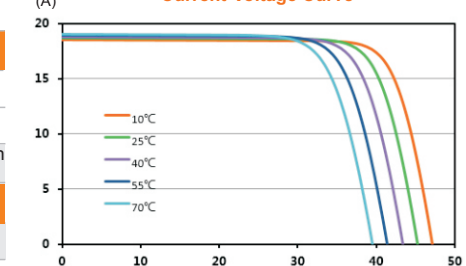
Current-Voltage Curve
